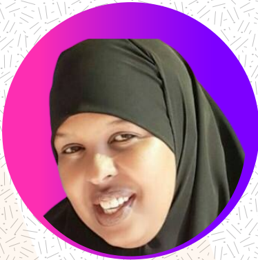
FATHIYA MAHBUB 40.6%
