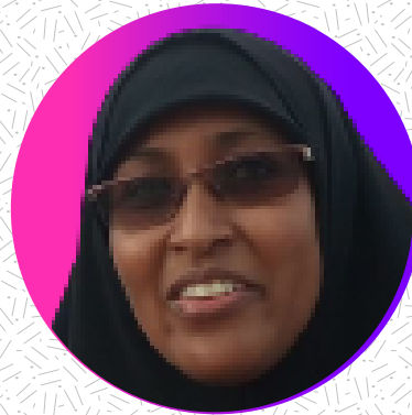
UBAH GEDI 23.0%
